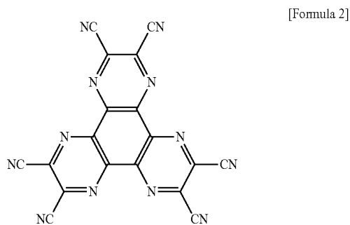
Synthesis Example
